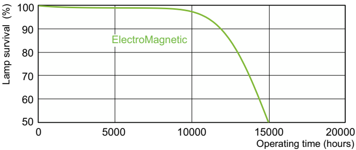
Life Expectancy Diagram - TL-D 15W/54-765 1SL/50
