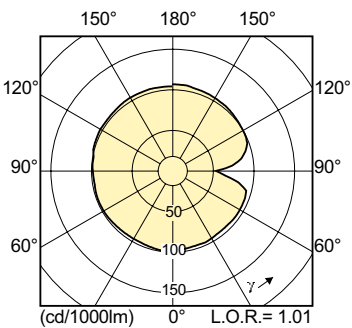
Light Distribution Diagram - MST CosmoWhite CPO-TT Xtra 60W/628 E27
