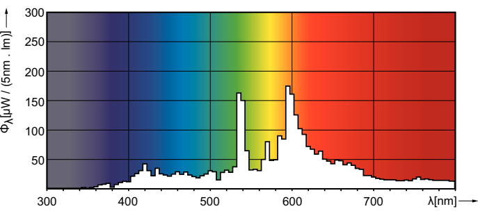
Spectral Power Distribution Colour - MASTERC CDM-TD 70W/830 RX7s 1CT/12
