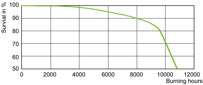
Life Expectancy Diagram - MASTERC CDM-R 35W/830 E27 PAR20 30D 1CT
