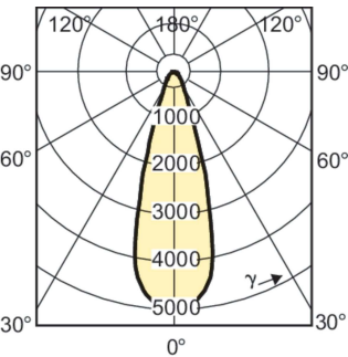
Light Distribution Diagram - MASTERC CDM-R 35W/830 E27 PAR20 30D 1CT
