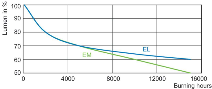
Lumen Maintenance Diagram - MASTER CDM-TP 70W/830 PG12-2 1CT/12
