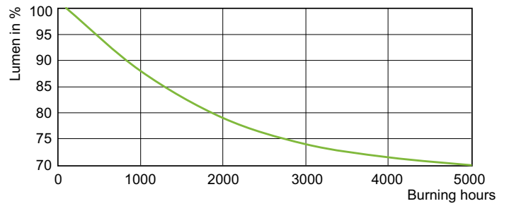
MHN-SA 2000 W Lumen Maintenance 400 V XW
