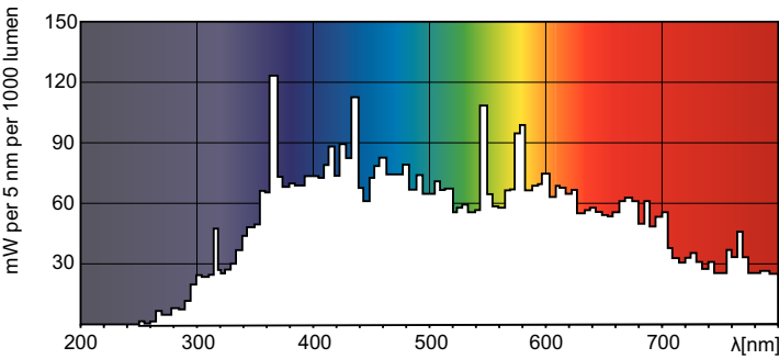
Spectral Power Distribution Colour - MSR 1200 HR 1CT/2
