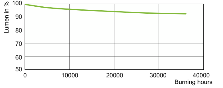
Lumen Maintenance Diagram - MST SON-T PIA Plus 150W/220 E40 - 1SL/12
