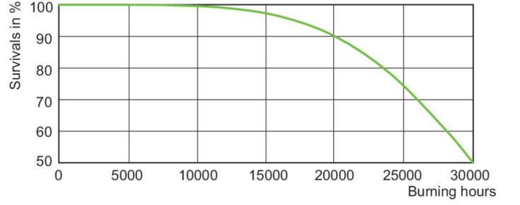
Life Expectancy Diagram - MST SON-T PIA Plus 70W/220 E27 1SL/12
