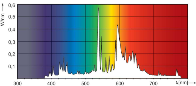
Spectral Power Distribution Colour - MASTER CityWh CDO-ET Plus 100W/828 E40
