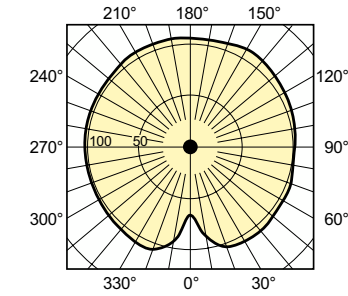
Light Distribution Diagram - MST SON-T PIA Plus 600W/220 E40 1SL/12
