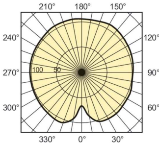
Light Distribution Diagram - MASTER GreenPower CG T 400W E40 1SL/12
