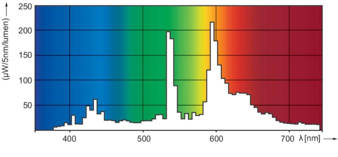
Spectral Power Distribution Colour - CDM-Rm Elite Mini 20W/830 GX10 MR16 40D
