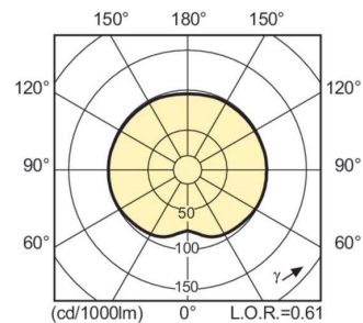
Light Distribution Diagram - MASTERC CDM-TC Elite 70W/942 G8.5 1CT
