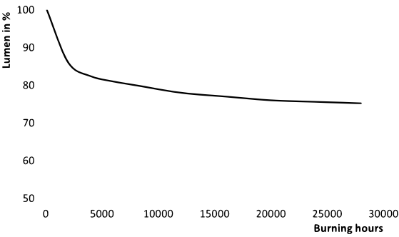
Lumen Maintenance Diagram - MSTSON-TPIA Plus 70W E27 1CT/12
