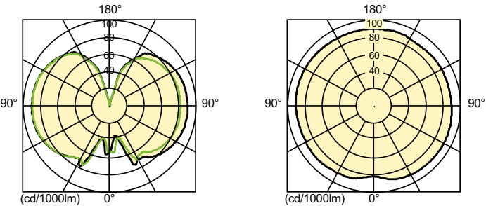
Light Distribution Diagram - CDM T9 ELITE 315W/930/U/E NA
