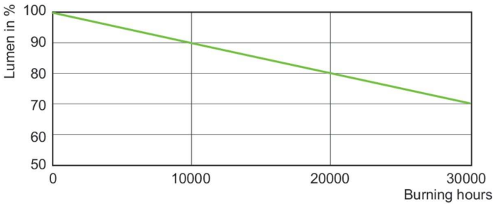
Lumen Maintenance Diagram - CDM T9 ELITE 315W/930/U/E NA
