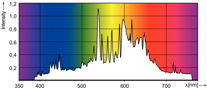
Spectral Power Distribution Colour - CDM T9 ELITE 315W/930/U/E NA
