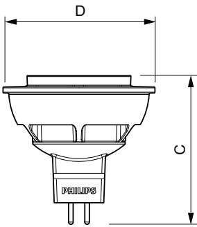
MR16 12V 7W-35W 24D 2700K GU5.3 Dimtone
