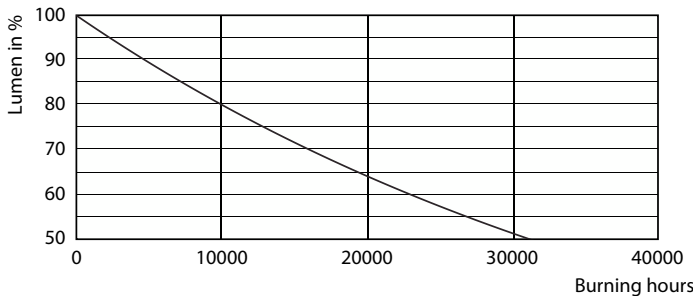
Lumen Maintenance Diagram - Corepro Lustre ND 5.5-40W E27 827 P45 CL
