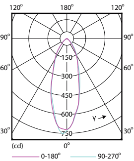
Light Distribution Diagram - Essential LED 4.6-50W GU10 830 36D
