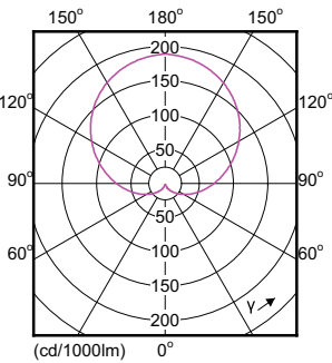
Light Distribution Diagram – LED Globe 60W G93 E27 WW FR ND 1CT/4
