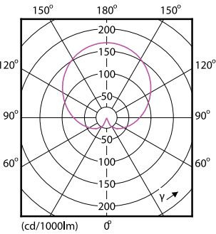
Light Distribution Diagram - CorePro LEDbulb ND 8-60W A60 B22 827
