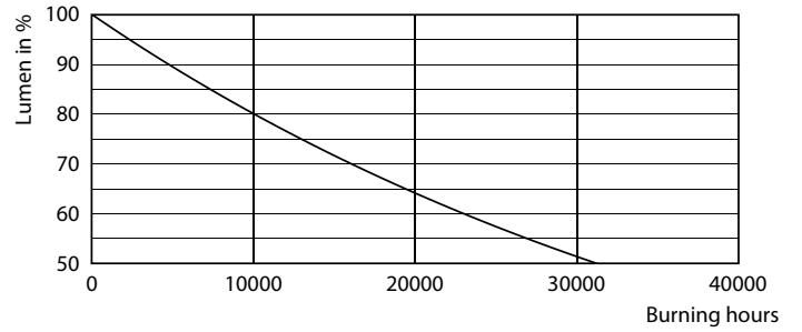
Lumen Maintenance Diagram - CLA LEDCandle ND 2-25W B35 E14 827 CL
