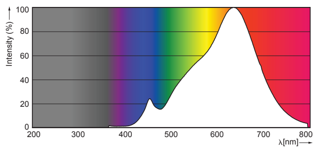
Spectral Power Distribution Colour - MAS LED MR16 ExpertColor 7.2-50W 927 10D
