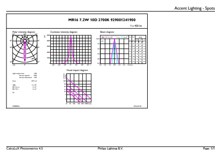
General uniform lighting - MAS LED MR16 ExpertColor 7.2-50W 927 10D
