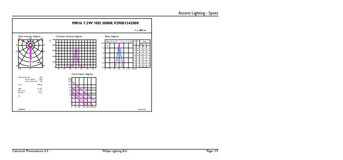
General uniform lighting - MAS LED MR16 ExpertColor 7.2-50W 930 10D
