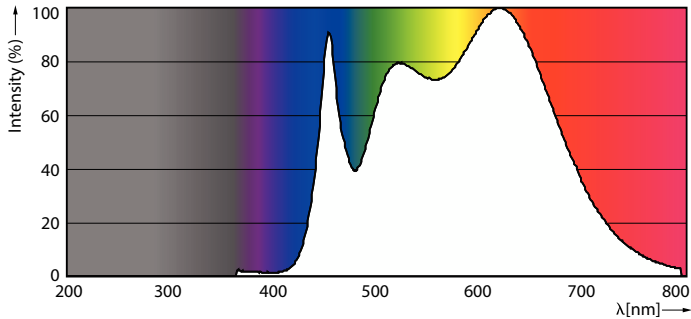
Spectral Power Distribution Colour - MAS LED MR16 ExpertColor 7.2-50W 940 10D
