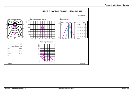
General uniform lighting - MAS LED MR16 ExpertColor 7.2-50W 930 24D
