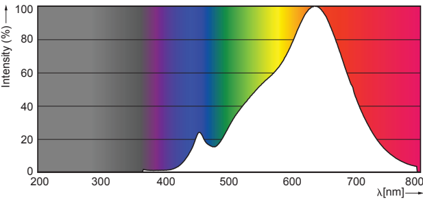
Spectral Power Distribution Colour - MAS LED MR16 ExpertColor 7.2-50W 927 36D
