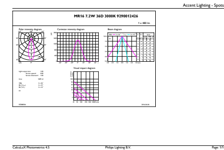
General uniform lighting - MAS LED MR16 ExpertColor 7.2-50W 930 36D
