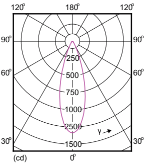
Light Distribution Diagram - MAS LED MR16 ExpertColor 8-50W 940 36D
