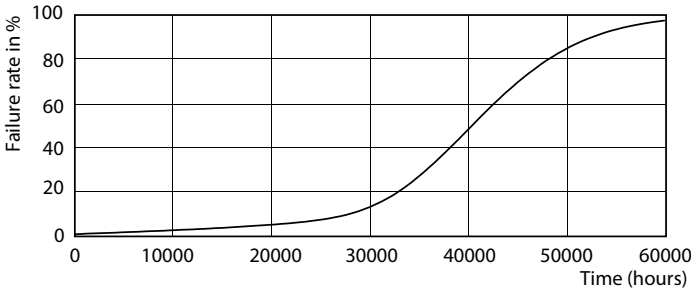
Life Expectancy Diagram - MAS LED MR16 ExpertColor 8-50W 940 36D
