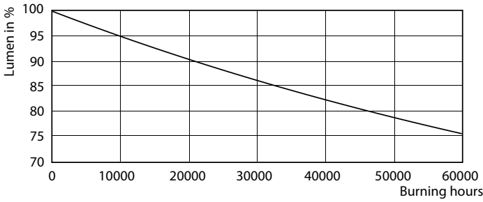
Lumen Maintenance Diagram - MAS LED MR16 ExpertColor 8-50W 940 36D
