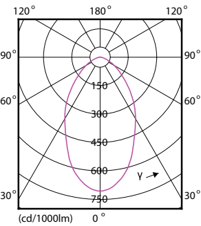
Light Distribution Diagram - 165HB/LED/740/ND NB DL 2/1
