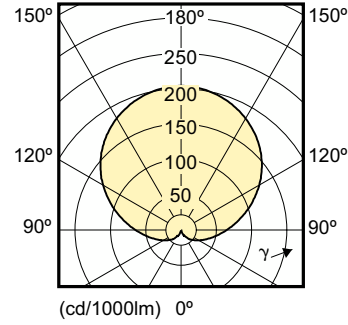
Light Distribution Diagram - ESS LEDBulb 8-48W E27 6500K 230V A60 TR
