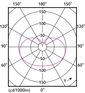
Light Distribution Diagram - LED classic 75W A60 E27 WW FR ND 1CT/10
