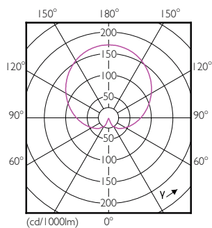
Light Distribution Diagram - CorePro LEDbulb ND 5-40W A60 E27 830
