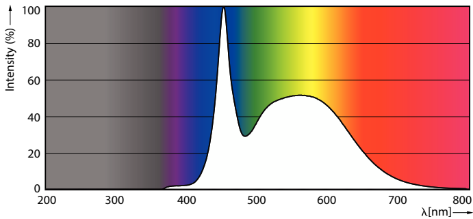
Spectral Power Distribution Colour - CorePro LEDbulb ND 12.5-100W A60 E27 865
