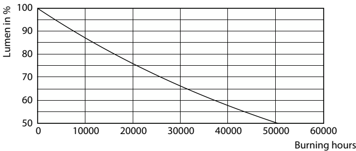
Lumen Maintenance Diagram - 5.5PAR16/AMB/F40/830/E26/DIM120V BC 1PK
