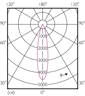
Light Distribution Diagram - MAS LEDspot D 13-100W E27 927 PAR38 25D
