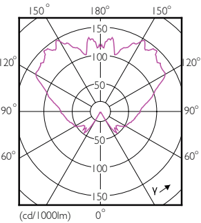
Light Distribution Diagram – Corepro candle ND 5.5-40W E27 827 B35 CL
