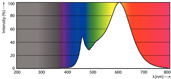
Spectral Power Distribution Colour - MAS LED spot VLE D 5.5-35W MR16 830 36D
