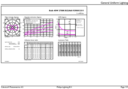
General uniform lighting - CLA LEDBulb D 5-40W A60 B22 827 CL
