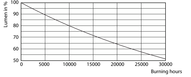
Lumen Maintenance Diagram - CorePro LED spot 2.6-20W 827 MR11 36D
