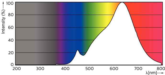
Spectral Power Distribution Colour - MAS LED ExpertColor 6.5-35W MR16 927 60D
