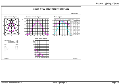
Accent Lighting Spots - MAS LED ExpertColor 6.5-35W MR16 927 60D
