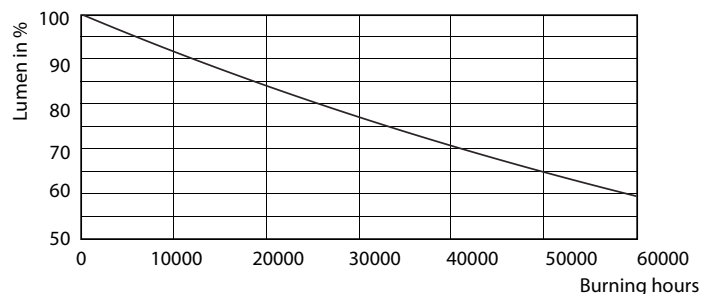
Lumen Maintenance Diagram - MAS LED ExpertColor 6.5-35W MR16 930 36D
