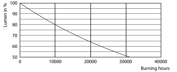
Lumen Maintenance Diagram - CLA LEDCandle ND 4.3-40W E14 827 B35 FR
