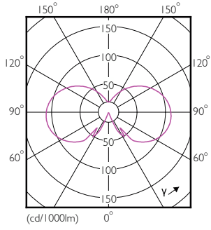
Light Distribution Diagram - CLA LEDCandle ND 4.3-40W E14 827 B35 FR
