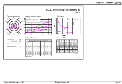
General uniform lighting - CLA LEDCandle ND 4.3-40W E14 827 B35 FR
