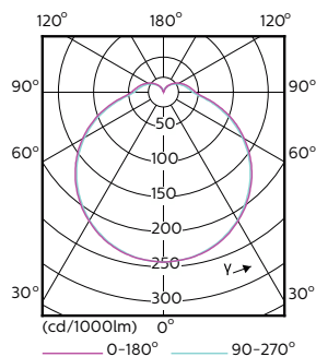
Light Distribution Diagram - CorePro LED PLC 4.5W 840 4P G24q-1
