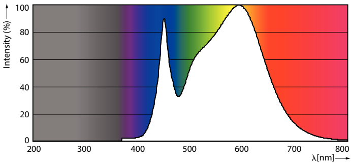
Spectral Power Distribution Colour - Master LED PAR30L 20W 15D 840 CN
