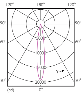
Light Distribution Diagram - Master LED PAR30L 20W 15D 840 CN
