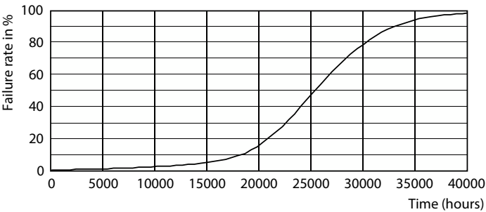
Life Expectancy Diagram - Master LED PAR30L 32W 30D 830
