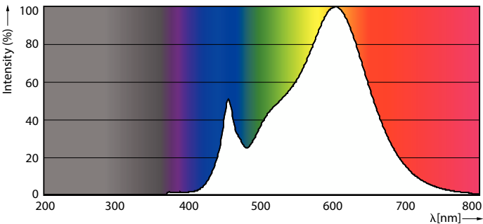
Spectral Power Distribution Colour - Master LED PAR30L 32W 30D 830
