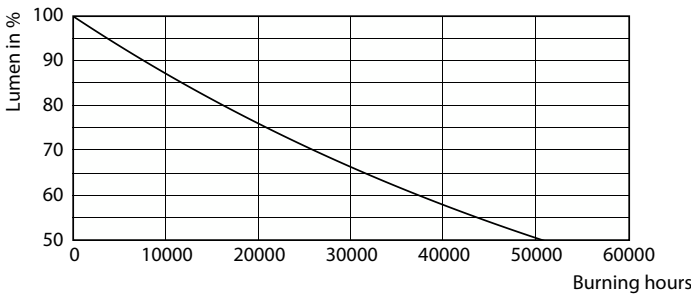
Lumen Maintenance Diagram - Master LED PAR30L 32W 30D 830
