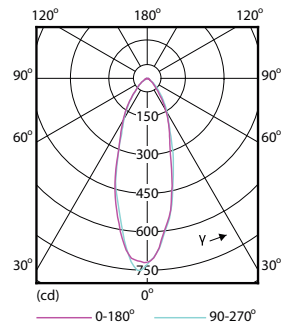
CorePro LEDspotMV 50W GU10 830 36D CLA
