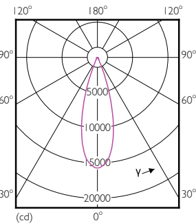
Light Distribution Diagram - Master LED PAR30L 40W 30D 840
