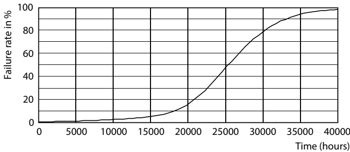
Life Expectancy Diagram - Master LED PAR30L 40W 30D 840
