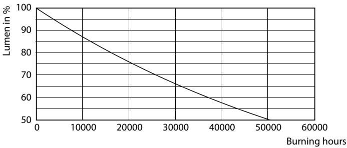
Lumen Maintenance Diagram - Master LED PAR30L 40W 30D 840
