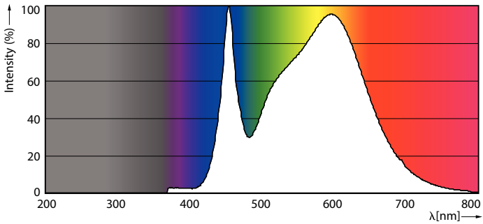
Spectral Power Distribution Colour - Master LED PAR30L 40W 30D 840
