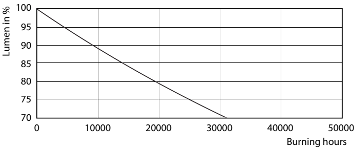
Lumen Maintenance Diagram - CorePro LEDtube 1200mm 16W830 G5 I APR
